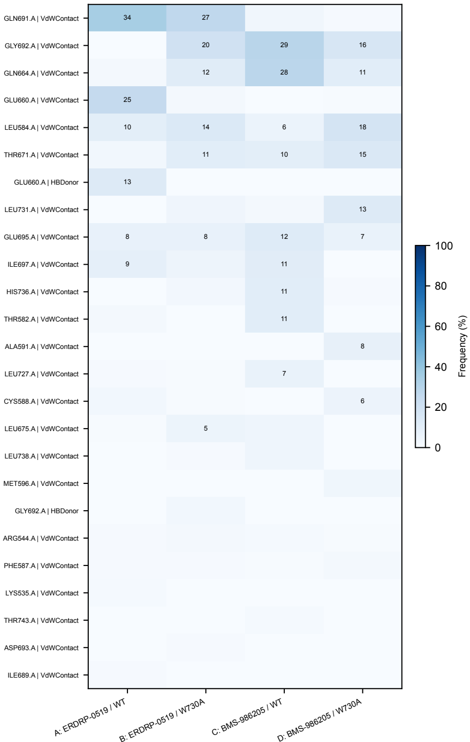
PLIF interaction frequencies — top 25 across all cases
